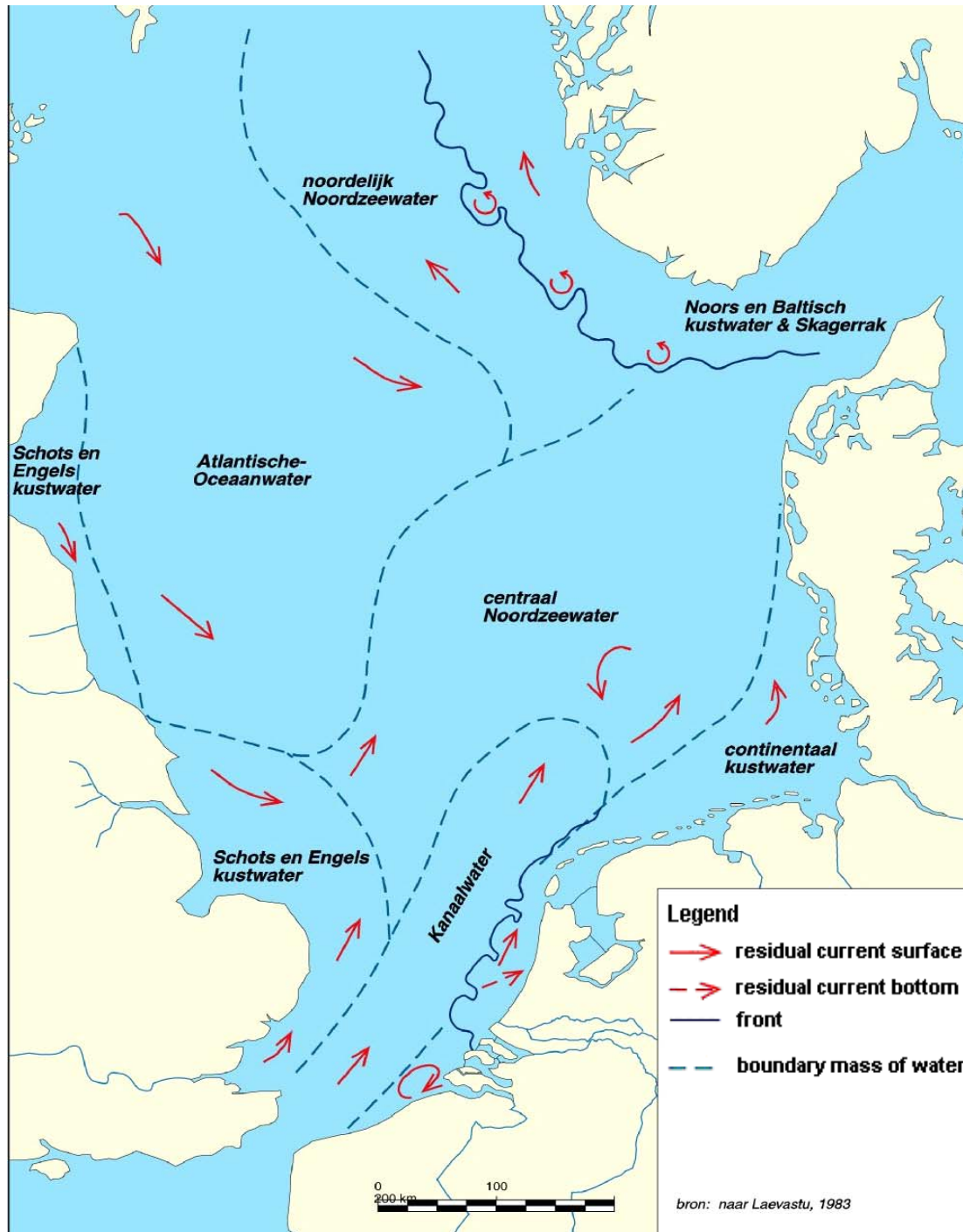
Figure 3 Flow patterns in the North Sea
