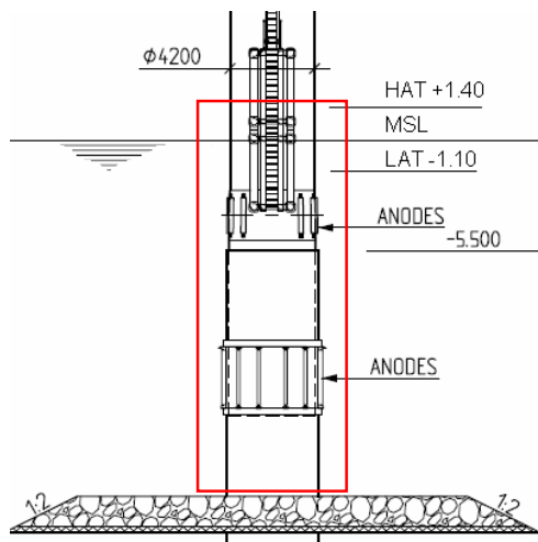
Figure 6 Schematic view on the submerged part of the monopile and OWEZ foundation. Monopile surface is to be monitored from the intertidal zone to the foundation, as indicated by the red line
