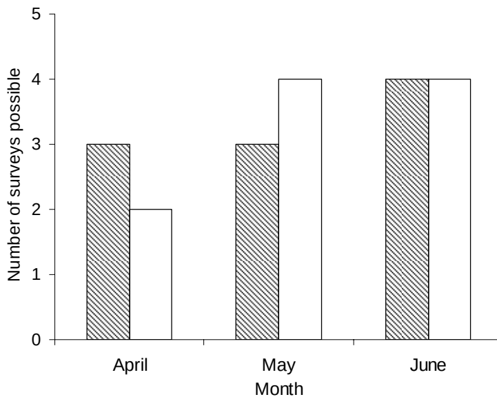
Figure 6.4. The maximum number of surveys possible in April, May and June of 2006 (hatched bars) and 2007 (empty bars), given wind speed and survey independence constraints.
