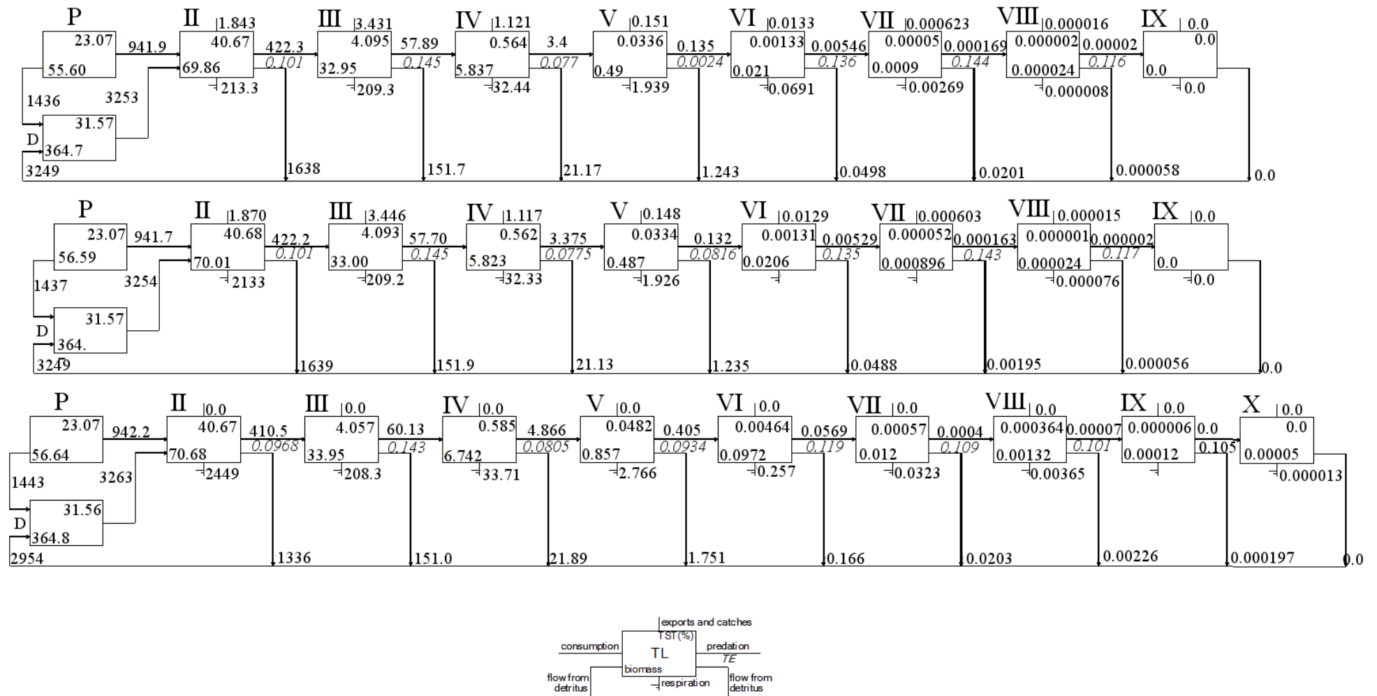
Figure 5.3 Lindeman spine diagrams of A = Scenario 1 (Business-as-usual), B= Scenario 2 (OWF installation), and C = Scenario 3 (OWF installation and fishing restrictions). TL = Trophic level, P = Producers, D = Detritus, TE = Transfer efficiency, TST = Total system throughput.
