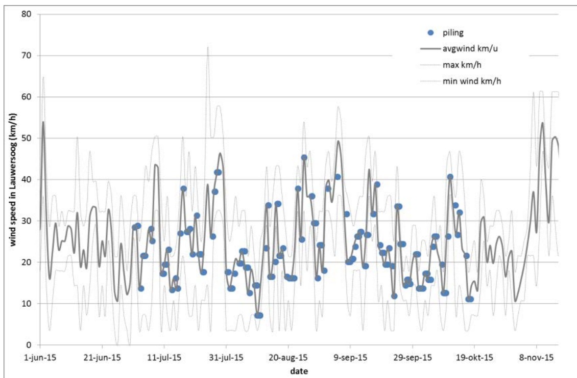
Figure 35. Wind speed (km/h) at Lauwersoog during the pile driving period. Individual pilling events are plotted as blue dots in the graph.
