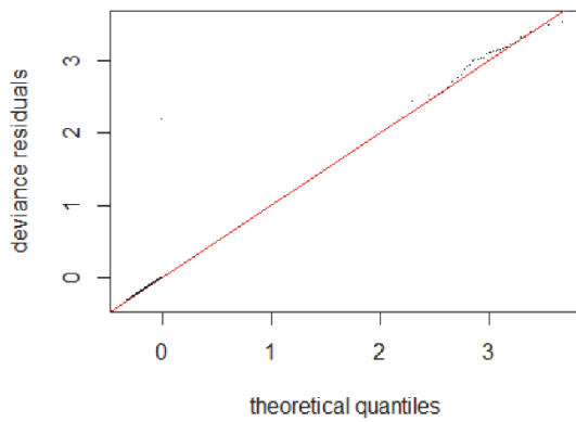
Q-Q plot
