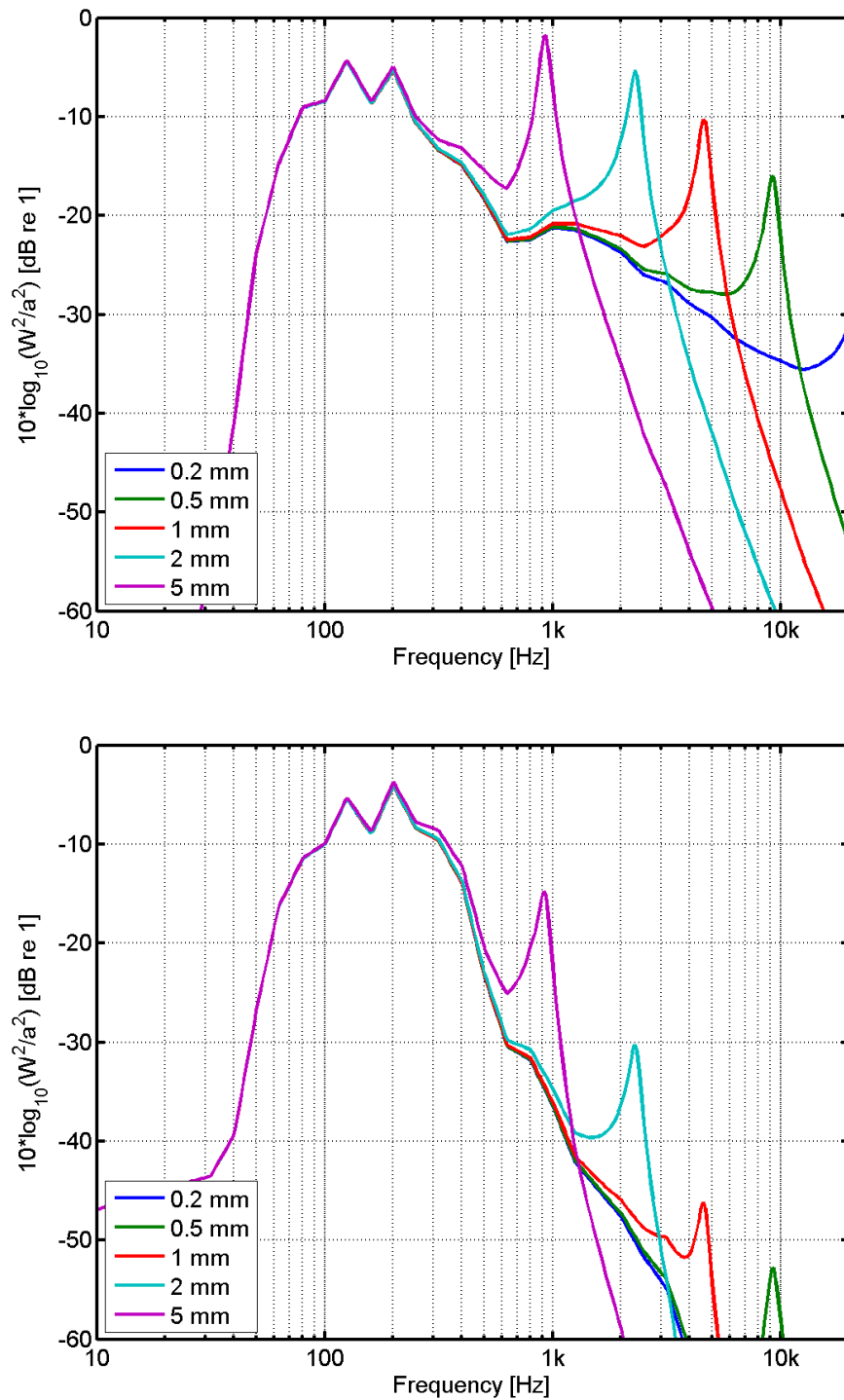
Figure 5. Forced response of air bubbles with different radii under influence of the sound pressure level spectrum of the OWEZ@100m signal, as measured in the field (top), and as measured in the larvaebriator during play-back of the filtered (50 Hz - 1 kHz) signal (bottom).
