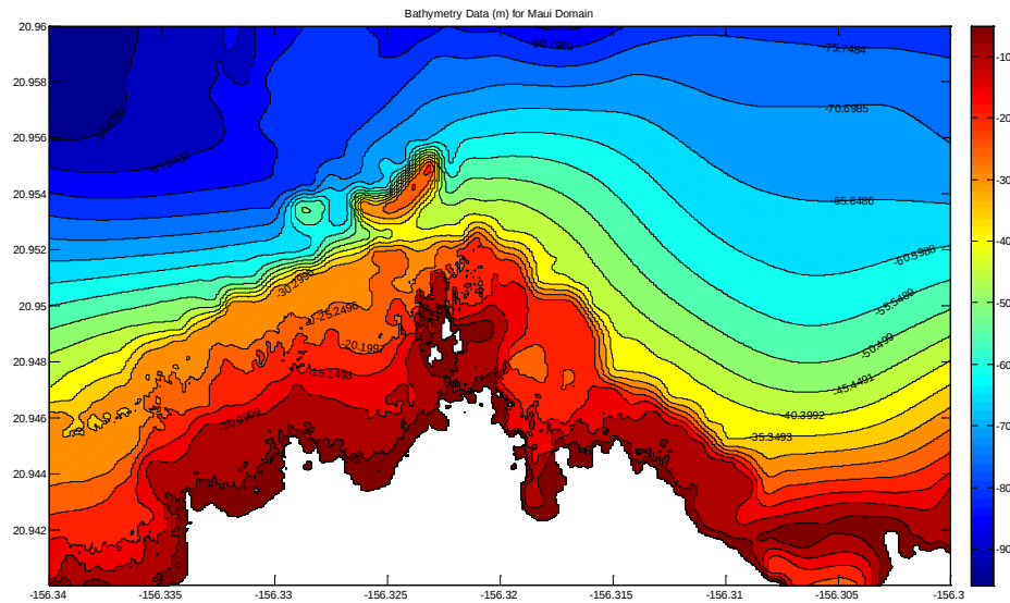
Bathymetry off Pa'uwela, Maui: Depth in meters supplied by HINMREC to OCEANLINX/MECO from LIDAR Data to be confirmed with Side Scan Sonar Survey
