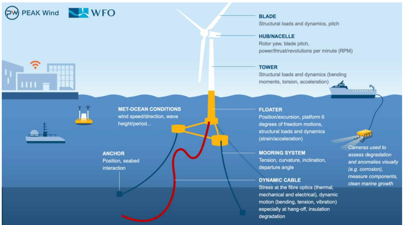
Figure 6. Summary of the information typically sought after in FOWT inspection and condition monitoring Source: PEAK Wind & WFO
