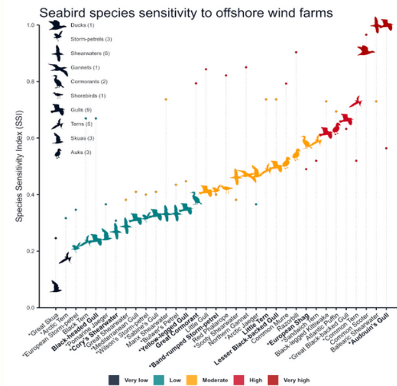
Figure 1: Seabird species sensitivity to marine wind farms (from Guilherme et al., 2023). Closed circles show the vulnerability score (VS), i.e., the highest value between the rescaled (i.e., range 0-1) Collision Vulnerability (CV) and Displacement Vulnerability (DV); silhouettes show the Species Sensitivity Index (SSI), i.e., the highest value between the rescaled Collision Sensitivity Index (CSI) and Displacement Sensitivity Index (DSI). The 34 seabird species are scored into five categories of sensitivity (very low; low; moderate; high; very high), according to their VS (closed circles) or their SSI (silhouettes). The categories of sensitivity are set on a comparative basis between species. Species names with an asterisk (*) have CSI > DSI . Species with regular breeding populations along the Portuguese mainland coast are in bold. Number of species per taxonomic group in brackets.
