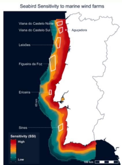
Figure 2: Seabird sensitivity to marine wind farm expansion in Portugal (from Guilherme et al., 2023). Seabird sensitivity to marine wind farm expansion in Portugal was calculated using density-distribution maps (ind. per 4×4 km grid cells) across the seasons of the year each species occurs in Portugal (Meirinho), and a Species Sensitivity Index (SSI) estimated using species-specific factors related with species' vulnerability to collision with, and displacement due to disturbance from marine wind farms. For each of the 34 species, we multiplied the natural log of the density in each grid cell by the respective SSI value. The final map was obtained by summing the values in each cell across species (see Methods). Isolines delineate five categories of sensitivity: low (dark blue) to very high (dark red). Boundaries of proposed wind farm sites are in white (the Aguçadoura site is a pilot marine wind farm in operation from 2020).
