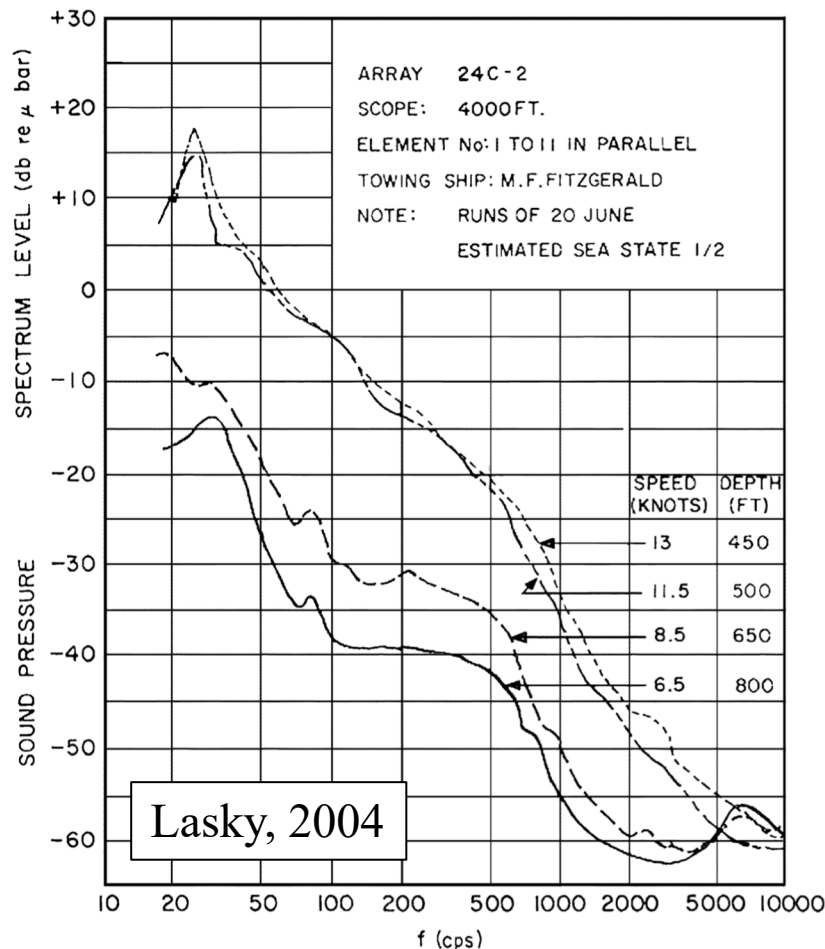
Fig. 11. Effect of speed on background noise for of 11-element array at 4000-foot cablescope.
