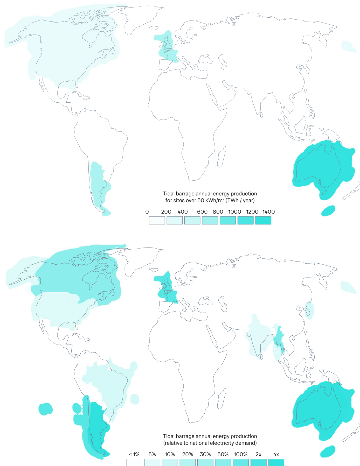
Figure 5 - Global annual energy potential from tidal range, in absolute terms (top) and relative to current national electricity demand (bottom).
