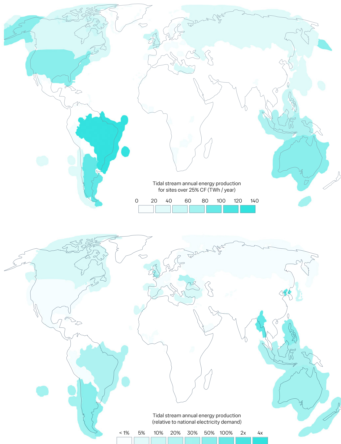
Figure 1 – Global annual energy potential from tidal stream, in absolute terms (top) and relative to current national electricity demand (bottom).
