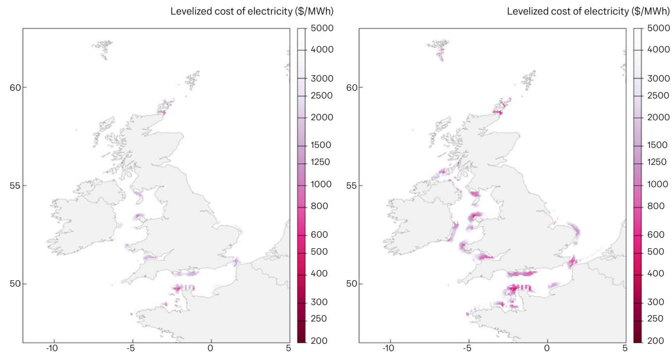
Figure 3 – Levelized cost of electricity from tidal stream across the UK, modelled using capacity factors from the 2 MW MCT machine (left) and the 1 MW TTS machine designed for medium-speed (right).
