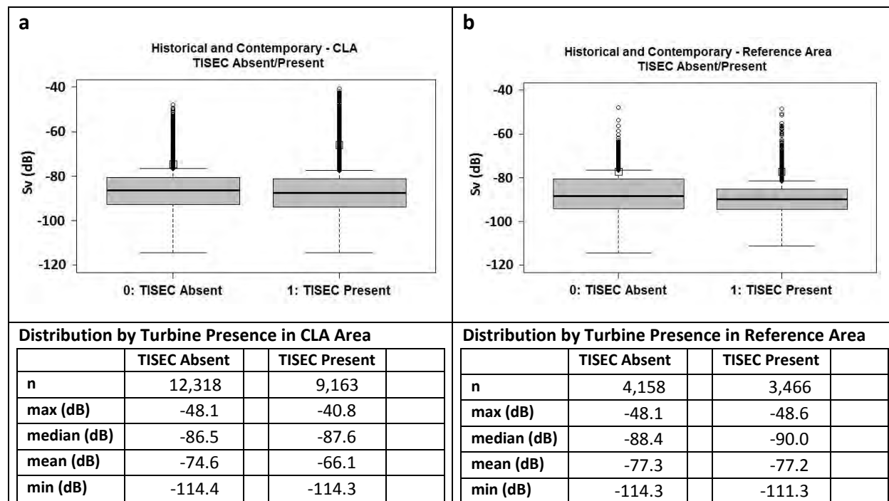
Figure 8. Distribution of S_v values without and with a TISEC device in CLA. S_v distributions and distribution statistics for both the (a) CLA and (b) Reference study areas are shown. Data shown are the data exported from Echoview (excluding zeros) integrated over the full water column binned in 20-m along-shiptrack horizontal bins. See text for description of boxplot.
