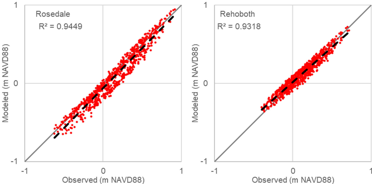
Figure 4-6: Modeled Versus Observed Water Levels
