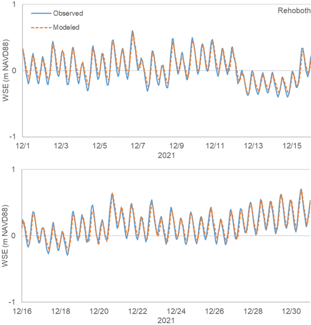
Figure 4-5: Observed and Modeled Water Levels at Dewey Beach, Rehoboth Bay
