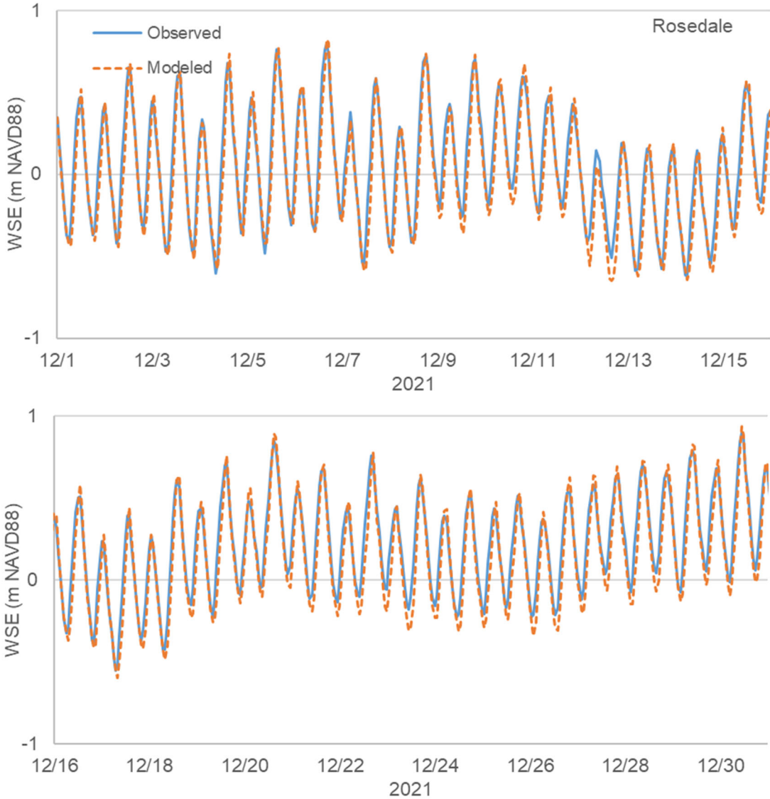
Figure 4-4: Observed and Modeled Water Levels at Rosedale Beach, Indian River Bay
