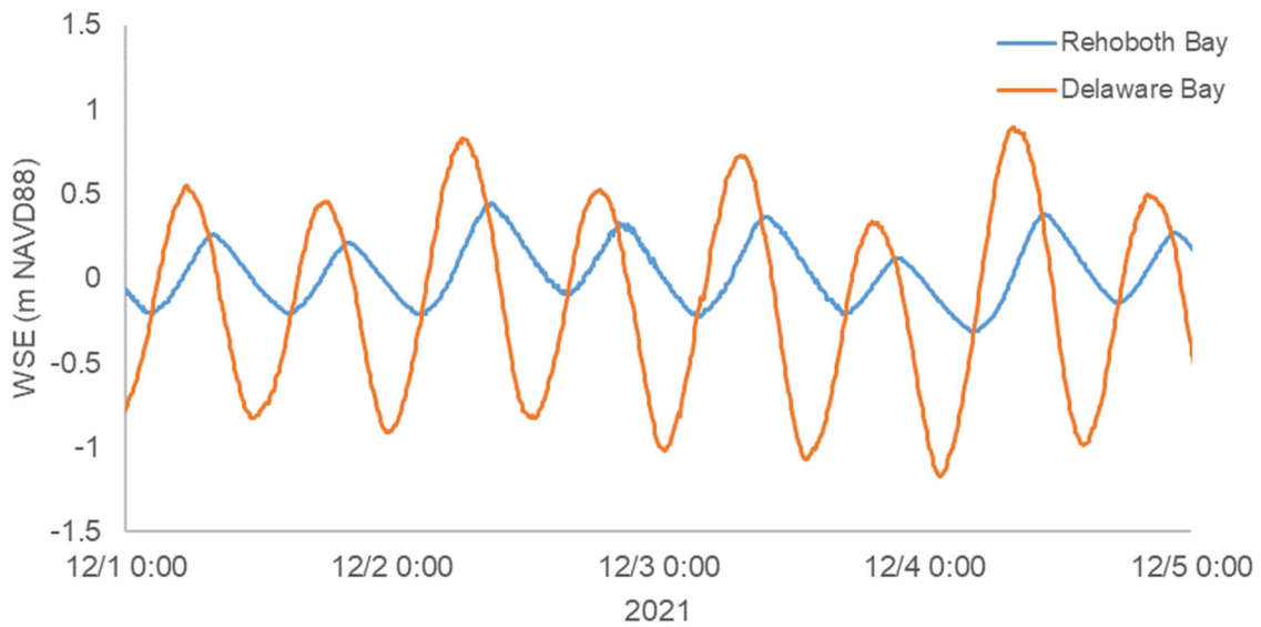
Figure 4-2: Observed WSE at Rehoboth Bay and Delaware Bay (Lewes)
