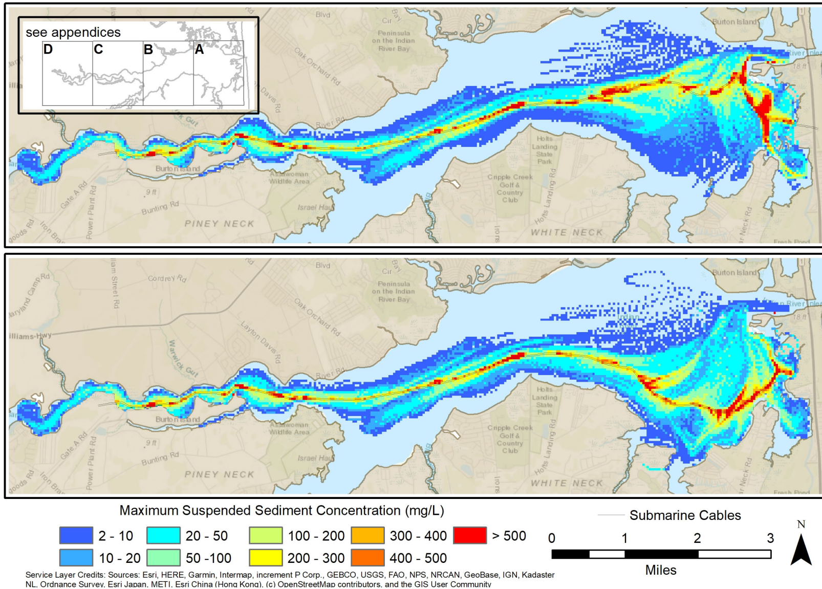
Figure 5-1: Modeled Predicted Maximum Suspended Sediment Concentrations
