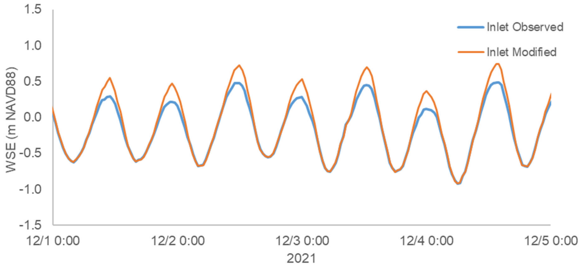
Figure 4-1: Observed WSE and Modified WSE for Tidal Boundary at Indian River Bay Inlet
