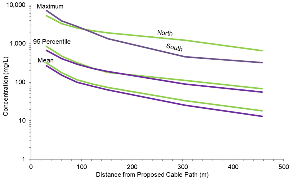
Figure 5-2: Predicted Suspended Sediment Concentration versus Distance from Cables
