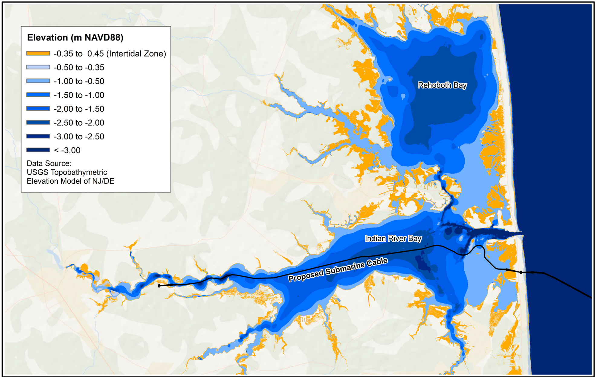
Figure 5: Indian River Bay and Rehoboth Bay Bathymetry
