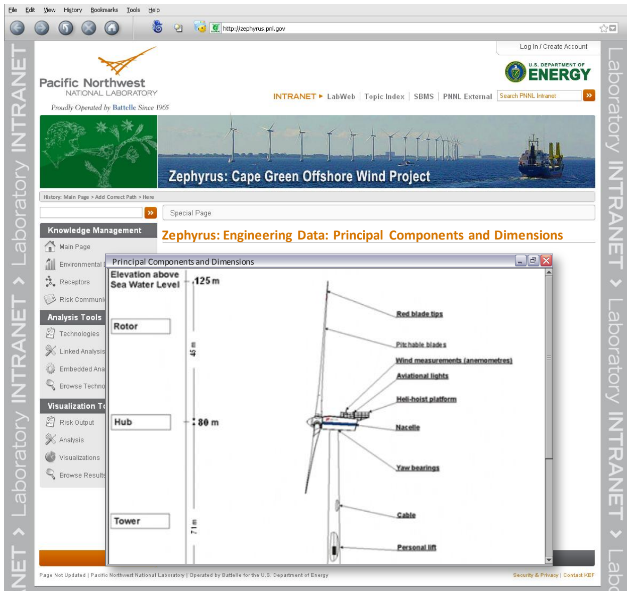
Figure 5. Engineering data on the principal components and dimensions of offshore wind turbine generator technology (2 – 4 MW).
