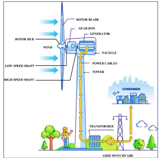
FIGURE 9. Different parts of wind turbine [116].
