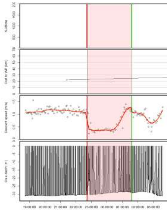
Figure 4.5. Example of a typical response to pile driving: grey seal hg43LZ-Z066-14, approximately 23 km away from Borkum Riffgrund (Monopole DE 610, unmitigated), revealed a rapid decline in descent speed when pile-driving commenced (3rd panel, left). During the last phase of pile-driving the, the descent speed returned to presumably normal levels. Note that very few GPS location fixes are available, insufficient to plot the track of the seal before, during and after pile driving.
