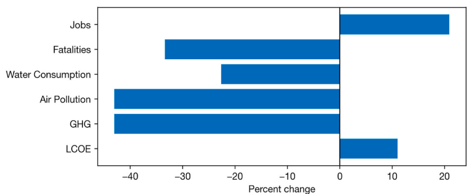
Fig. 9. Percent change in six sustainability metrics from low installed offshore wind capacity (1600 MW) to high (10000 MW).
