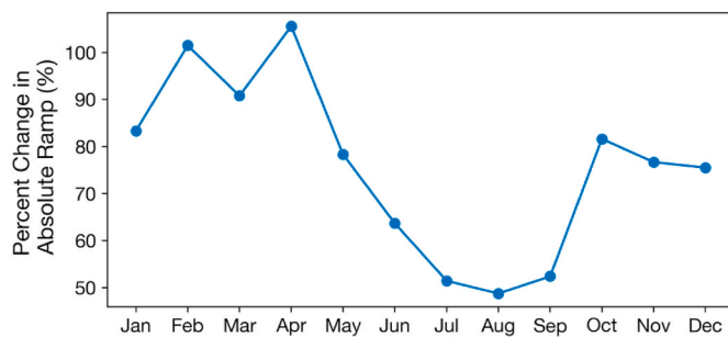
Fig. 7. Percent change in average absolute hourly hydropower ramp from 1600 MW to 10,000 MW of offshore wind capacity.
