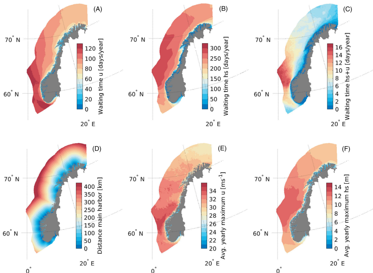
FIGURE A4 Data fields for the criteria under the met-ocean category. (A) Wind speed ( u ) accumulated (AWT) waiting time (days/year) where the wind speed exceeds 12 m/s with a time duration of >8\text{ h} ; (B) AWT of significant wave height ( hs ) exceeding 2 m lasting more than 8 h; (C) AWT time of hs + u , where u > 12\text{ m/s} and hs > 2\text{ m} lasting more than 24 h; (D) distance (km) to the closest major port; (E) the average yearly maximum of hourly wind speed ( u ); (F) the average yearly maximum of hourly significant wave height ( hs )
