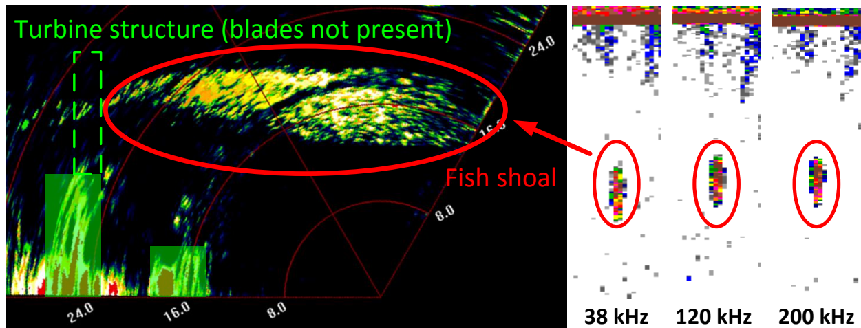
Figure 2 The multibeam swath shows a large fish shoal moving from left to right, tracked over 12 seconds. The turbine structure is outlined in green. The turbine blades were not fitted but their expected radius is outlined in dashed-green. The same target is detectable using the EK60 (shown on the right), where the frequency response can be used to aid target identification [4].
